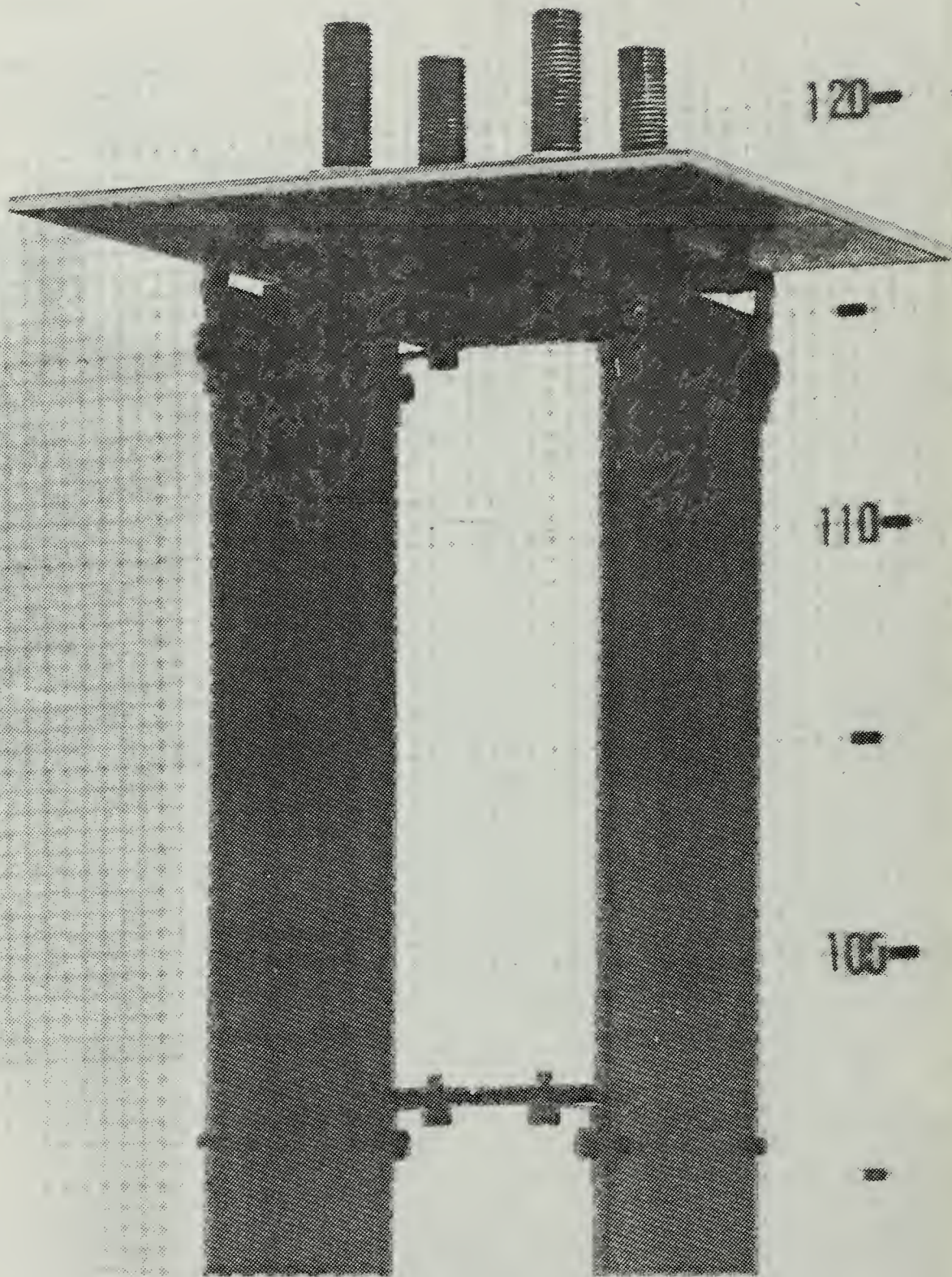
Figure 4. Flexible Manipulator Showing Transverse Bridges, Tip Loading and Grid Background.
