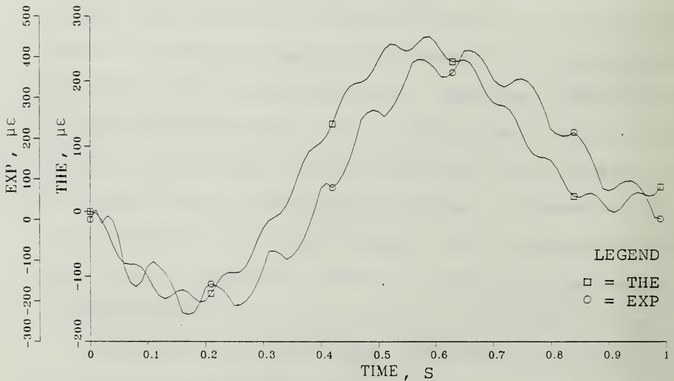
Figure 10. Microstrain for 2.115 Kg Load.
