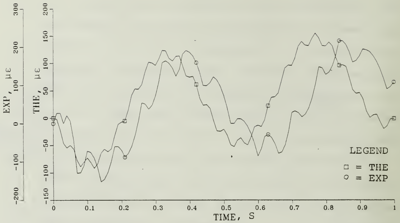
Figure 9. Microstrain For No Load.
