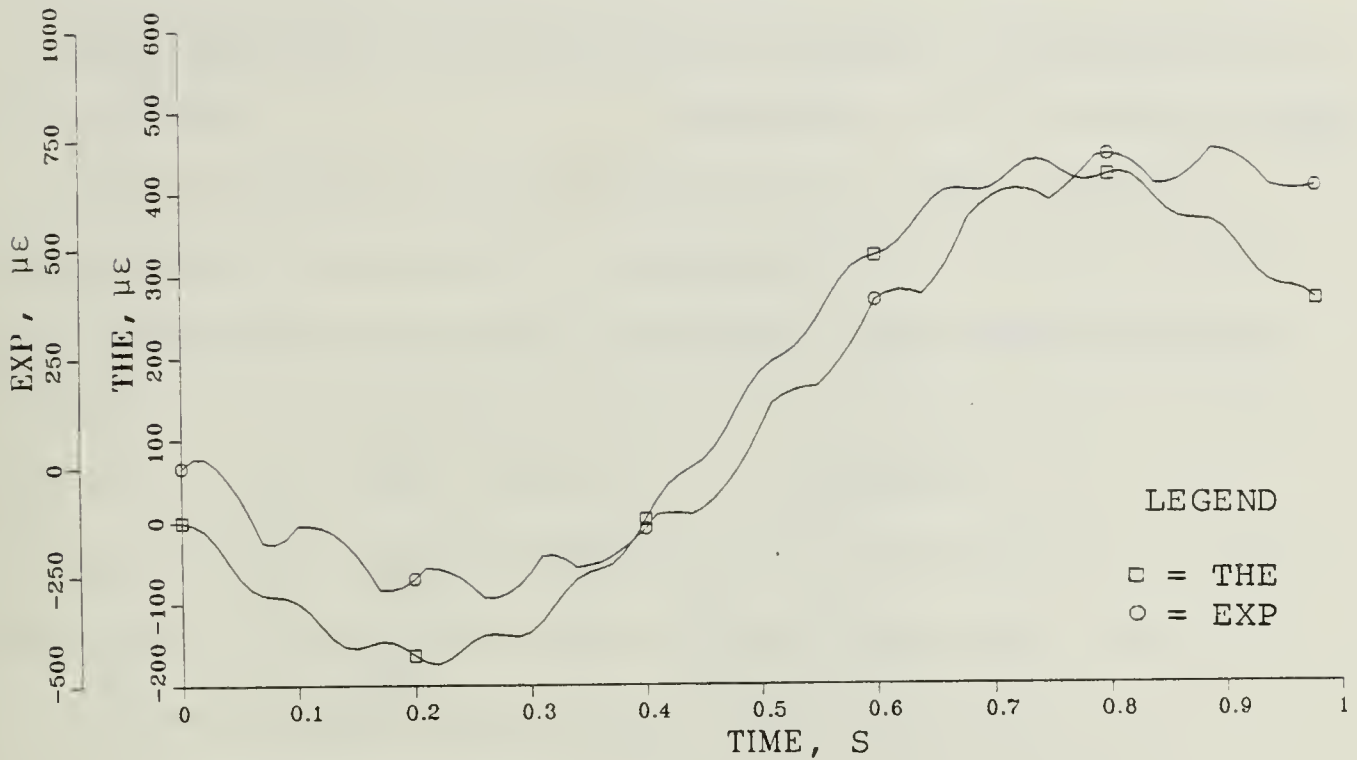
Figure 11. Microstrain For 4.23 Kg Load.
